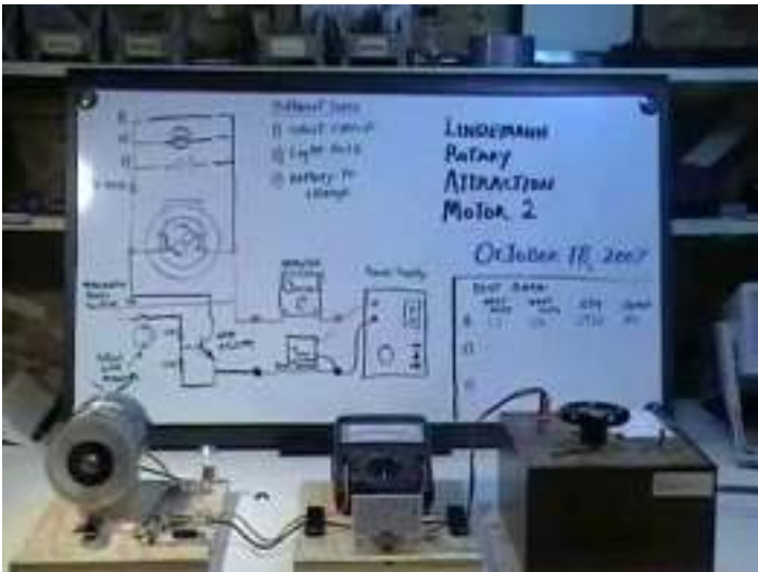
Figure 11.8 Lindemann Rotary Attraction Motor
