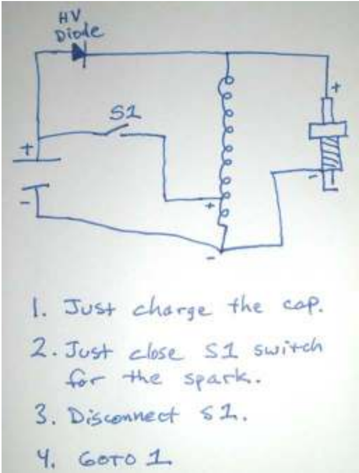
Figure 11.10 Water Spark Plug Circuit
