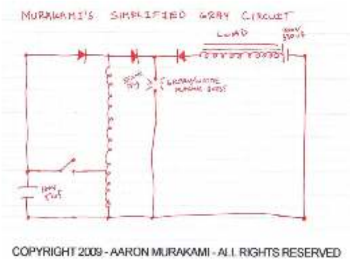
Figure 11.17 Murakami Simplified Gray Circuit
